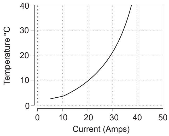
Temperature/Current Correlation Curve
